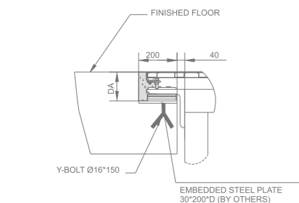
U/D SUPPORT DETAIL (SYMMETRIC)
